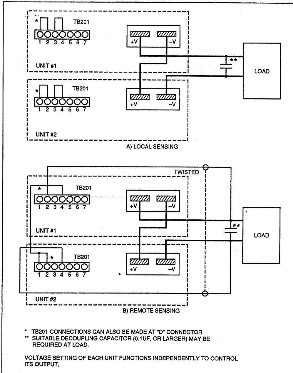
FIGURE 7: SERIES OPERATION
