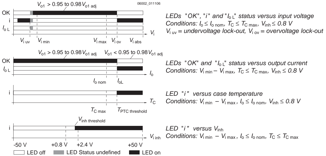
Fig. 23 LED indicators
