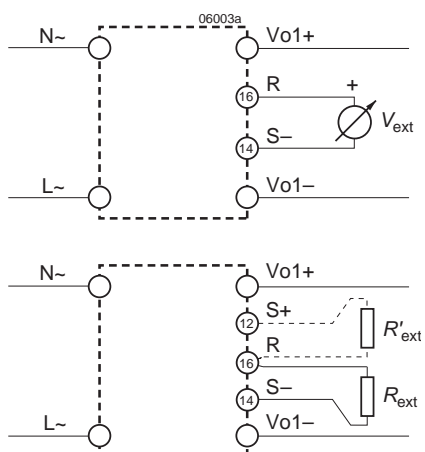
Fig. 21 Output voltage control for single-output models
