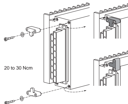
Connector retention brackets CRB HKMS
