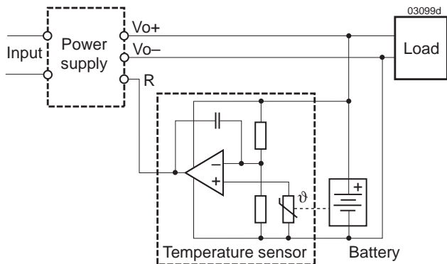
Fig. 24 Connection of a temperature sensor
