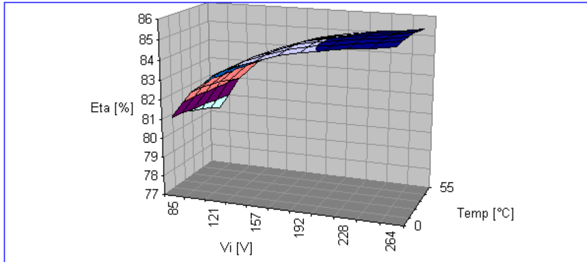
Figure 2. Efficiency vs. Input Voltage and Ambient Temperature, I_o = I_{o\text{nom}}
