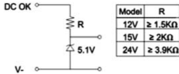
(a)5V signal
