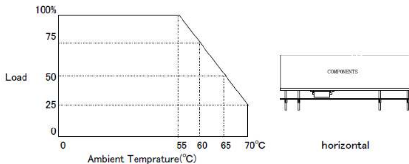
FIG.1 Derating Curve (Load vs Ambient Temp.)
