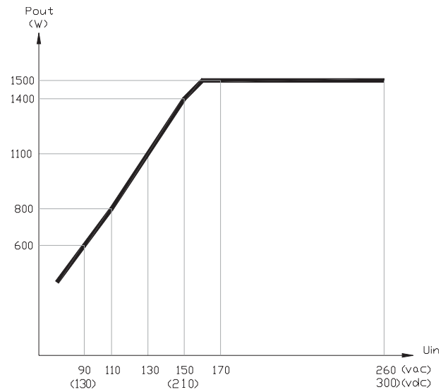
output power vs. input voltage derating curve
