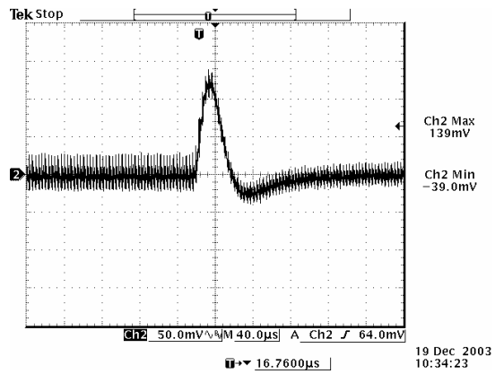
Transients 100% to 50% load 0.9 Vdc output
