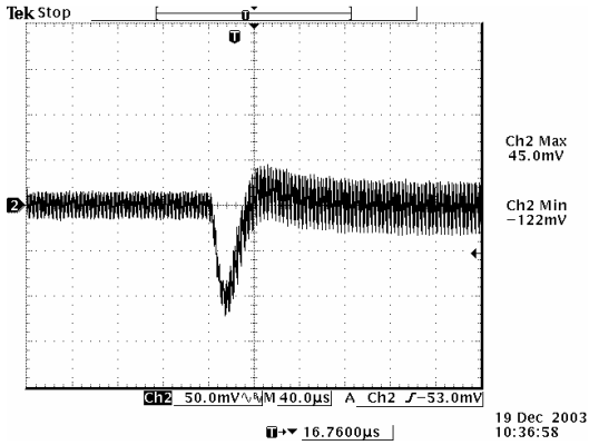
Transients 50% to 100% load 1.8 Vdc output
