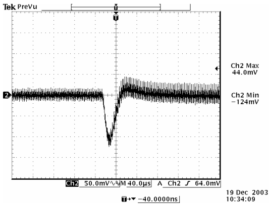
Transients 50% to 100% load 0.9 Vdc output
