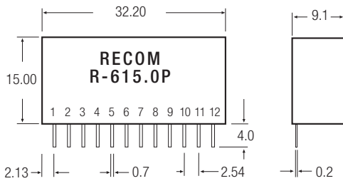
SIP12 PIN Package
