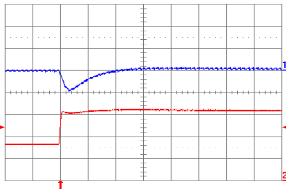
Fig. 1.5V.6: Output voltage response for V_{out} = 1.5\text{ V} to positive load current step change from 8 A to 16 A with slew rate of 5\text{ A}/\mu\text{s} at V_{in} = 12\text{ V} . Top trace: output voltage (200 mV/div.); Bottom trace: load current (5 A/div.). C_o = 100\ \mu\text{F} ceramic. Time scale: 20 \mu\text{s} /div.
