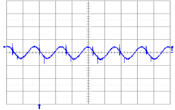
Fig. 2.0V.5: Output voltage ripple (20 mV/div.) at full rated load current into a resistive load with external capacitance 100 \mu\text{F} ceramic and V_{in} = 12 V for V_{out} = 2.0 V. Time scale: 2 \mu\text{s} /div.
