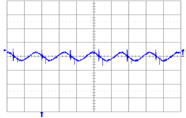
Fig. 1.5V.5: Output voltage ripple (20 mV/div.) at full rated load current into a resistive load with external capacitance 100\ \mu\text{F} ceramic and V_{in} = 12\text{ V} for V_{out} = 1.5\text{ V} . Time scale: 2 \mu\text{s} /div.
