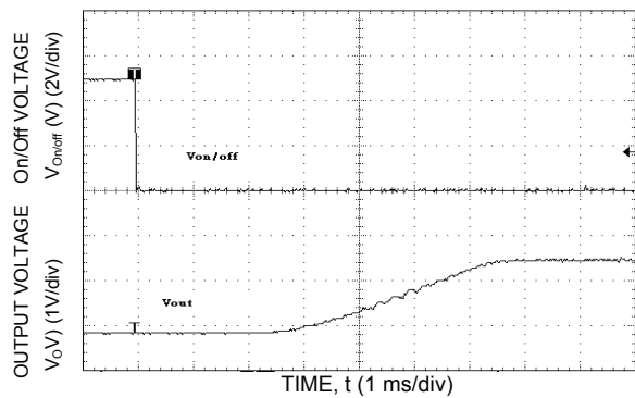
Figure 15. Typical Start-Up Using Remote On/Off with Low-ESR external capacitors ( 7 \times 150\ \mu\text{F} Polymer) ( V_{in} = 12\text{Vdc} , V_o = 3.3\text{Vdc} , I_o = 5.0\text{A} , C_o = 1050\ \mu\text{F} ).
