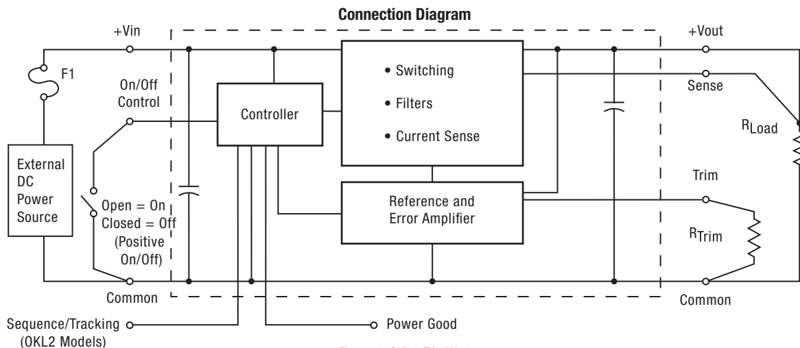
Figure 1. OKL2-T/6-W12
