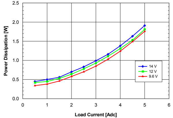
Fig. 2.0V.4: Power Loss vs. load current and input voltage for V_{out} = 2.0V converter mounted vertically with air flowing from pin 5 to pin 1 at a rate of 200 LFM (1 m/s) and T_a = 25^\circ C .
