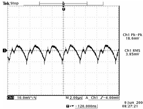
Ripple and noise at full load, 5.0 V input, 0.75 V output and T_a=25 degC
