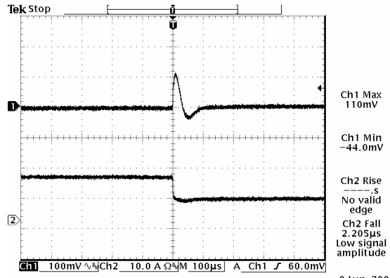
100% to 50% load step at V_{in}=5\text{ V} , V_o=0.75\text{ V}
