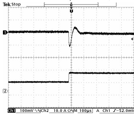
50% to 100% load step at V_{in}=5\text{ V} , V_o=3.3\text{ V}
