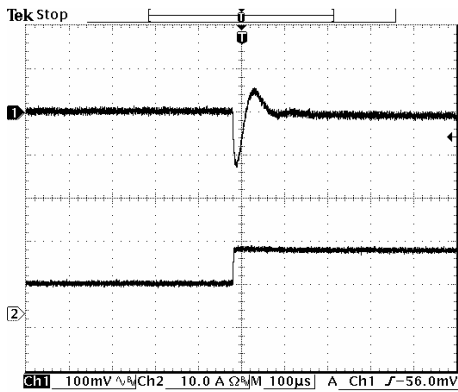
50% to 100% load step at V_{in}=5\text{ V} , V_o=0.75\text{ V}
