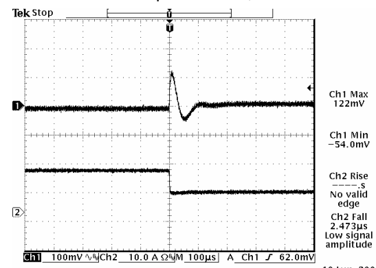
100% to 50% load step at V_{in}=5\text{ V} , V_o=3.3\text{ V}
