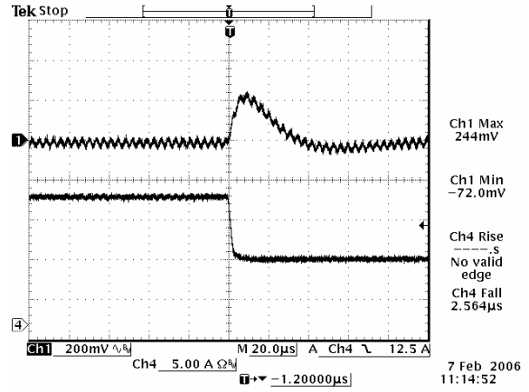
100% to 50% load Transient at 5.0 Vdc output
