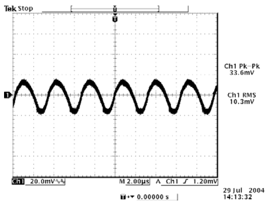
Ripple and noise at full load V_o=1.5 V
