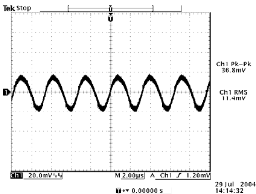
Ripple and noise at full load V_o=2.5 V
