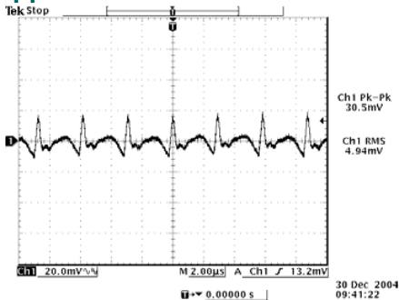
12 Vdc Input, 0.9 Vdc Output
