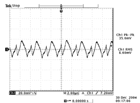
12 Vdc Input 3.3 Vdc Output
