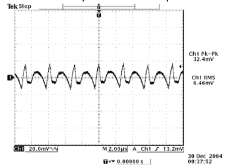
12 Vdc Input 1.8 Vdc Output
