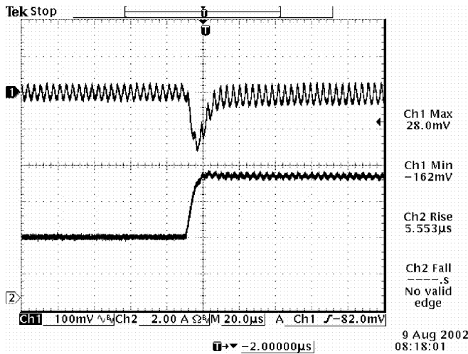
V_{out}=1.8\text{V} 50% to 100% load transients at 3.3V input and T_a=25^\circ\text{C}
