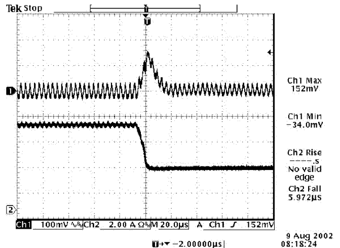
V_{out}=1.8\text{V} 100% to 50% load transients at 3.3V input and T_a=25^\circ\text{C}
