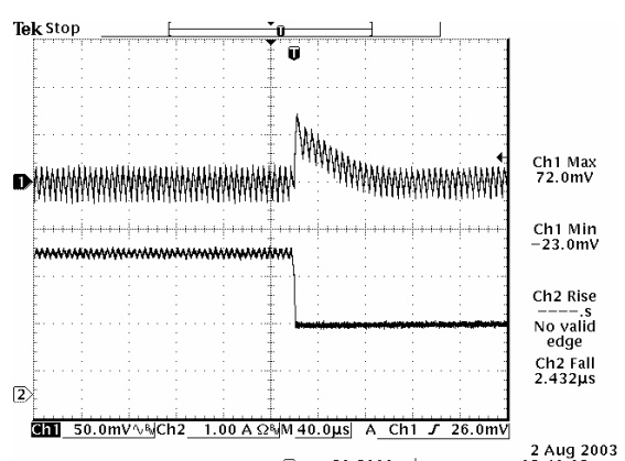
Transients 100% to 50% load 0.9 Vdc output
