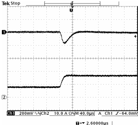
Transients 50% to 100% load 1.2 Vdc output
