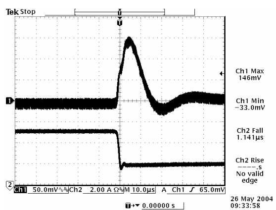
100% to 50% load step at V_{in}=5\text{ V} , V_o=1.2\text{ V}
