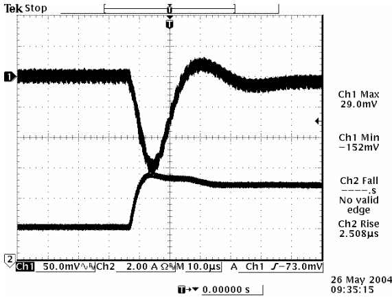
50% to 100% load step at V_{in}=5\text{ V} , V_o=0.75\text{ V}
