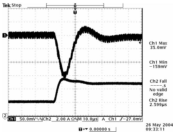
50% to 100% load step at V_{in}=5\text{ V} , V_o=1.2\text{ V}
