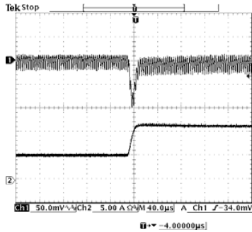
50% to 100% load 3.3 Vdc Input 1.2 Vdc Output
