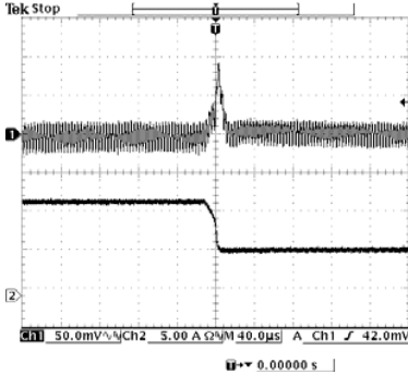
100% to 50% load 5 Vdc Input 1.8 Vdc Output
