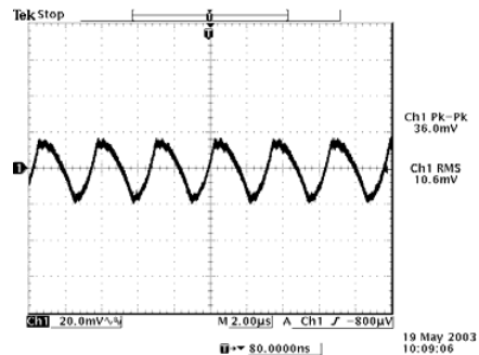
5 Vdc Input 1.8 Vdc Output
