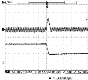
100% to 50% load 3.3 Vdc Input 1.5 Vdc Output
