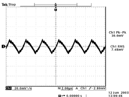
3.3 Vdc Input, 1.2 Vdc Output
