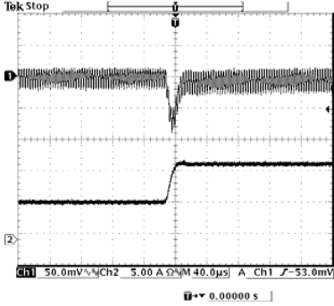
50% to 100% load 5 Vdc Input 1.8 Vdc Output
