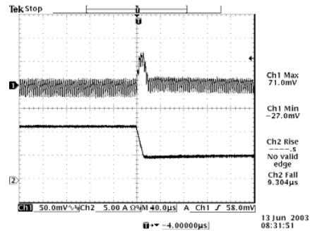
100% to 50% load 3.3 Vdc Input 1.2 Vdc Output
