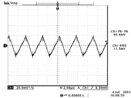
5 Vdc Input 2.5 Vdc Output
