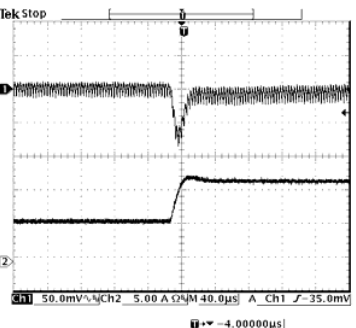
50% to 100% load 5 Vdc Input 1.0 Vdc Output
