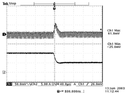
100% to 50% load 5 Vdc Input 1.2 Vdc Output
