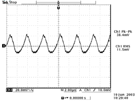
5 Vdc Input, 3.3 Vdc Output
