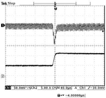
50% to 100% load 5 Vdc Input 1.5 Vdc Output
