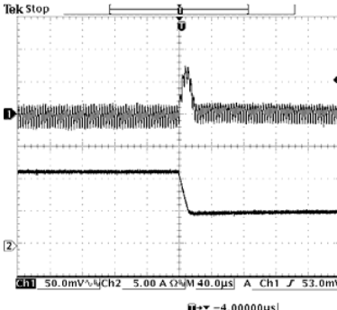
100% to 50% load 5 Vdc Input 1.5 Vdc Output
