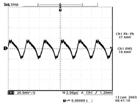
5 Vdc Input 1.5 Vdc Output
