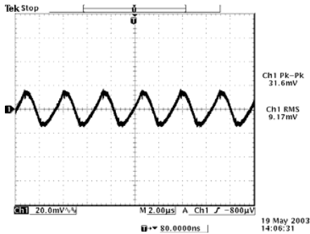
3.3 Vdc Input, 1.8 Vdc Output
