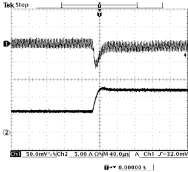
50% to 100% load 3.3 Vdc Input 1.8 Vdc Output
