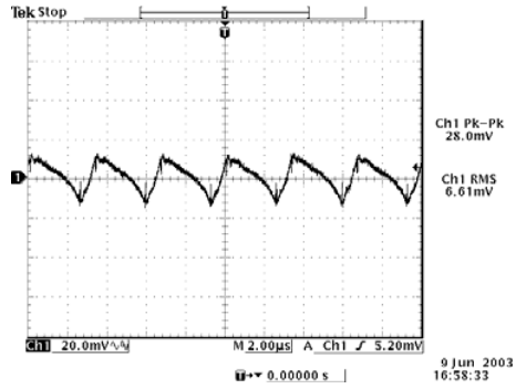
5 Vdc Input 1.0 Vdc Output
