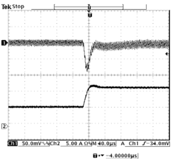
50% to 100% load 3.3 Vdc Input 1.0 Vdc Output
