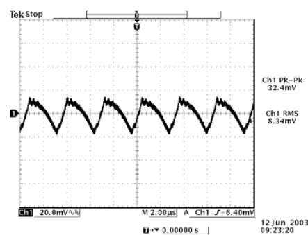
5 Vdc Input 1.2 Vdc Output
