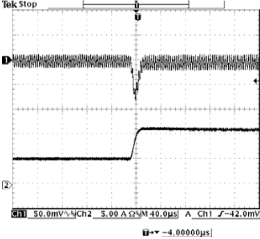
50% to 100% load 3.3 Vdc Input 1.5 Vdc Output
