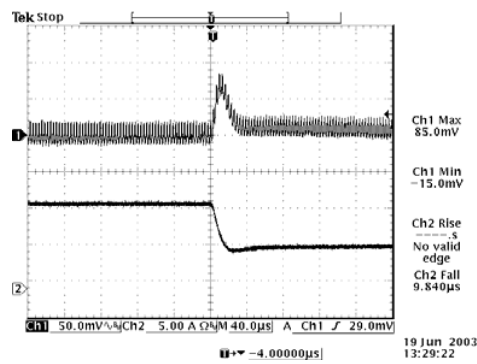
100% to 50% load 5.0 Vdc Input 3.3 Vdc Output
