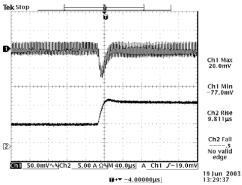
50% to 100% load 5.0 Vdc Input 3.3 Vdc Output
