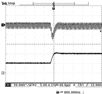
50% to 100% load 5 Vdc Input 1.2 Vdc Output
