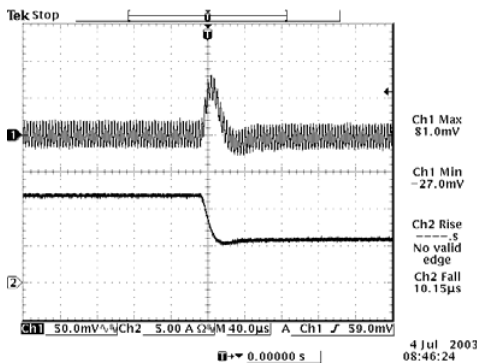
100% to 50% load 5.0 Vdc Input 2.5 Vdc Output
