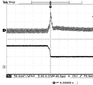
100% to 50% load 3.3 Vdc Input 1.8 Vdc Output
