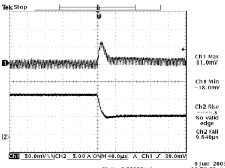
100% to 50% load 5 Vdc Input 1.0 Vdc Output
