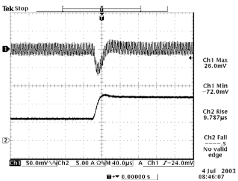
50% to 100% load 5.0 Vdc Input 2.5 Vdc Output
