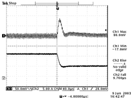
100% to 50% load 3.3 Vdc Input 1.0 Vdc Output
