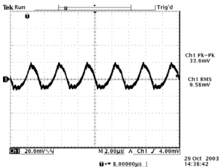
3.3 Vdc Input, 1.5 Vdc Output
