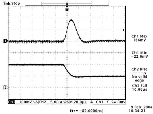
Transients 100% to 50% load 1.2 Vdc output
