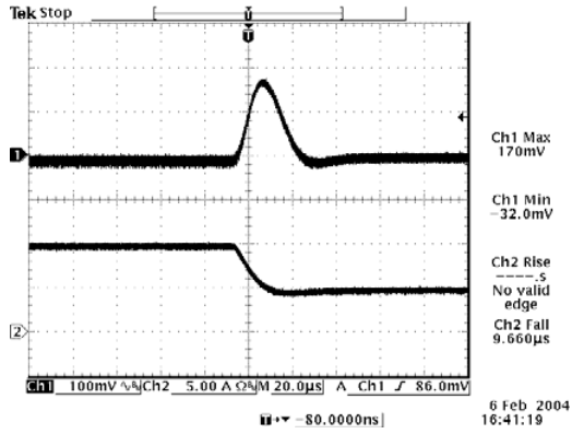
Transients 100% to 50% load 1.5 Vdc output
