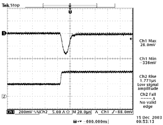
Transients 50% to 100% load 3.3 Vdc output
