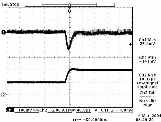
Transients 50% to 100% load 5.0 Vdc output
