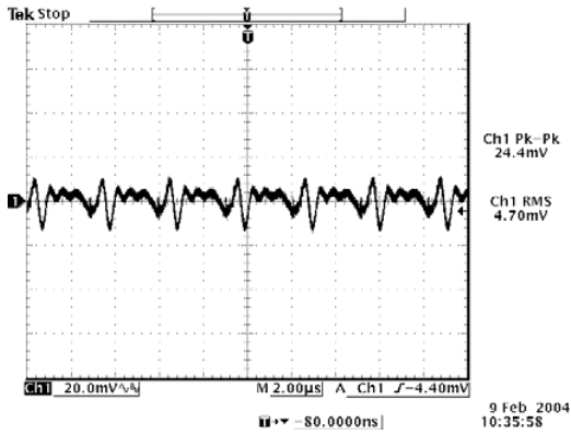
Ripple and noise at max load 1.2 Vdc output
