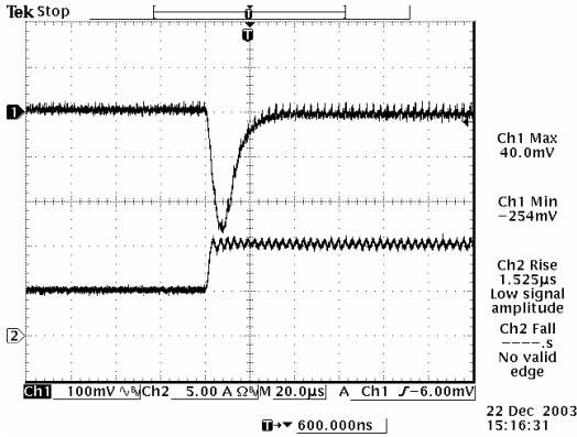
Transients 50% to 100% load 2.5 Vdc output
