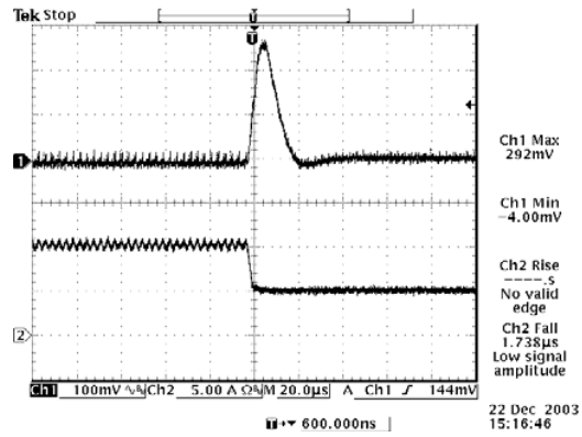
Transients 100% to 50% load 2.5 Vdc output
