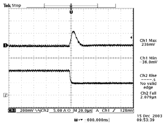
Transients 100% to 50% load 3.3 Vdc output
