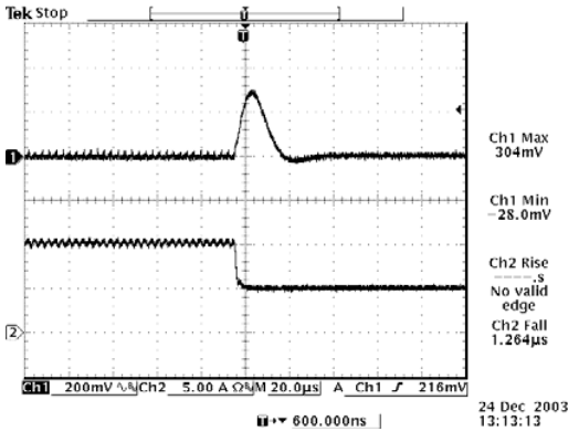
Transients 100% to 50% load 1.8 Vdc output
