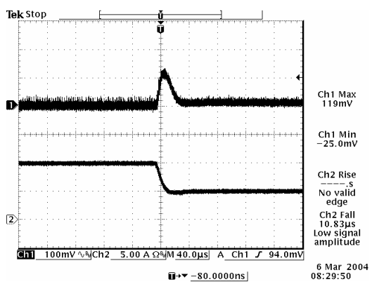
Transients 100% to 50% load 5.0 Vdc output
