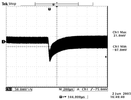
50% to 100% load transient at V_{in}=3.3 V, V_o=12 V
