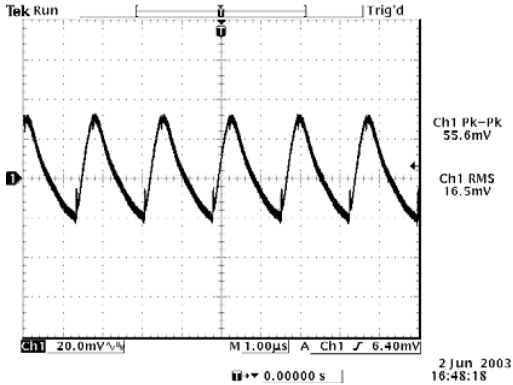
3.3 Vdc input, 12 Vdc output
