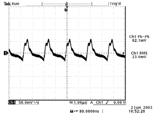
3.3 Vdc input, 15 Vdc output
