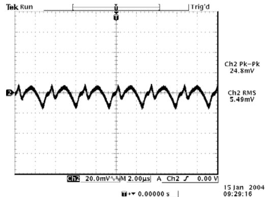
Ripple and noise at full load, V_{in}=5.0\text{ V} , V_o=1.2\text{ V}
