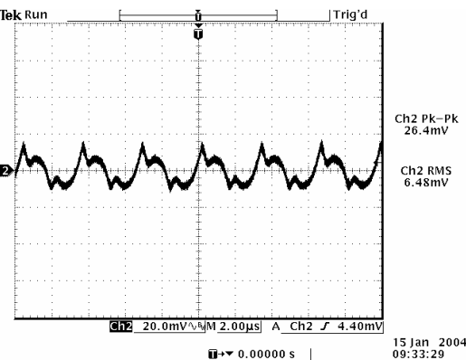
Ripple and noise at full load, V_{in}=5.0\text{ V} , V_o=2.5\text{ V}
