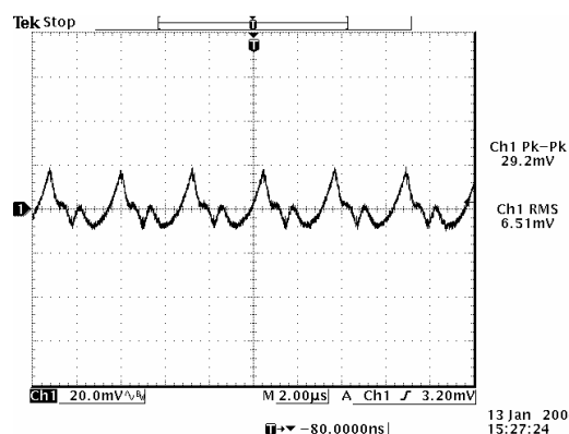
Ripple and noise at full load, V_{in}=5.0\text{ V} , V_o=3.3\text{ V}
