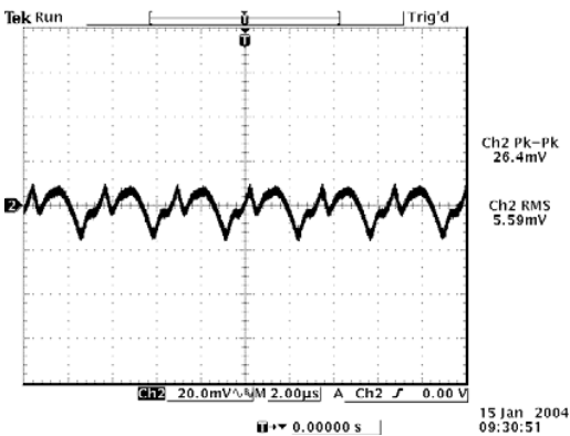
Ripple and noise at full load, V_{in}=5.0\text{ V} , V_o=1.5\text{ V}
