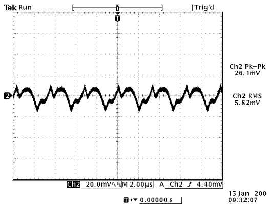
Ripple and noise at full load, V_{in}=5.0\text{ V} , V_o=1.8\text{ V}
