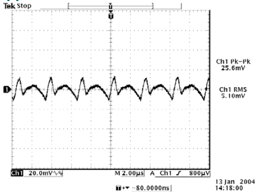
Ripple and noise at full load, V_{in}=5.0\text{ V} , V_o=0.7525\text{ V}
