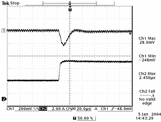
50% to 100% load step at V_{in}=12\text{ V} , V_o=2.5\text{ V}
