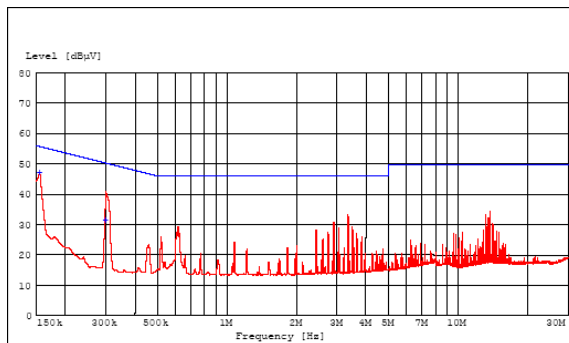
Figure 17. Typical Class B EMC signature of PIM300F with QBW025A0B1 module.
