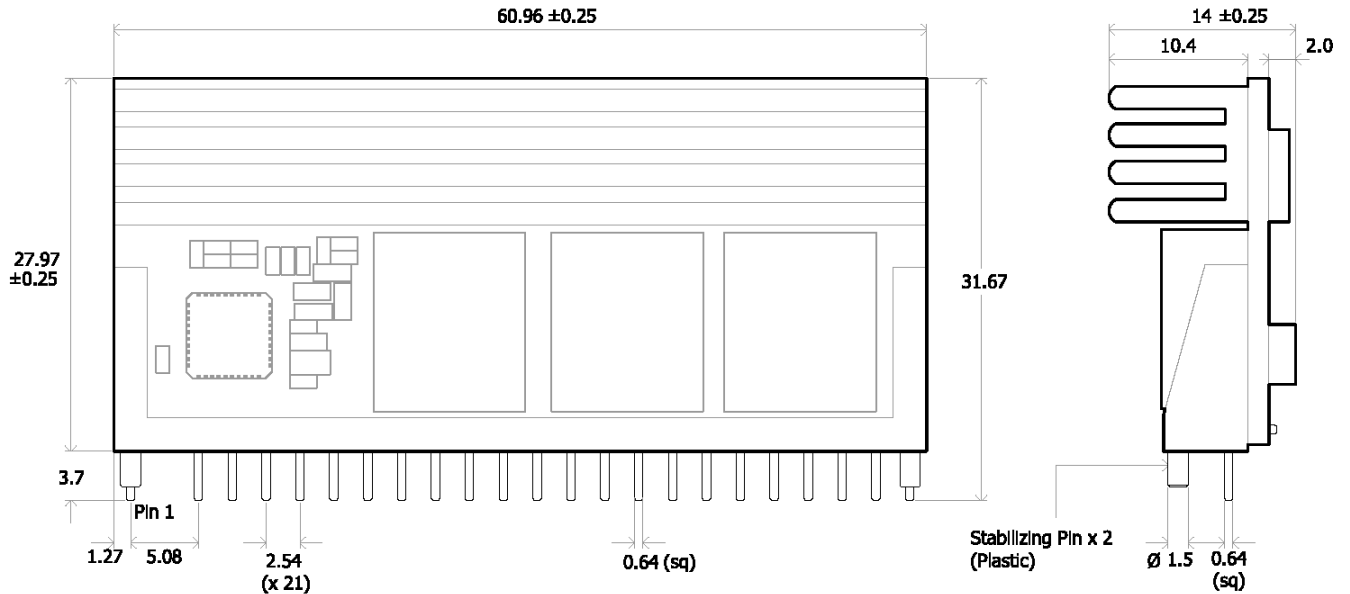
Figure 48. Mechanical Drawing
