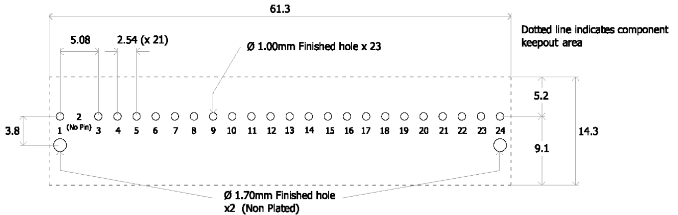
Figure 49. Recommended Footprint – Top View
