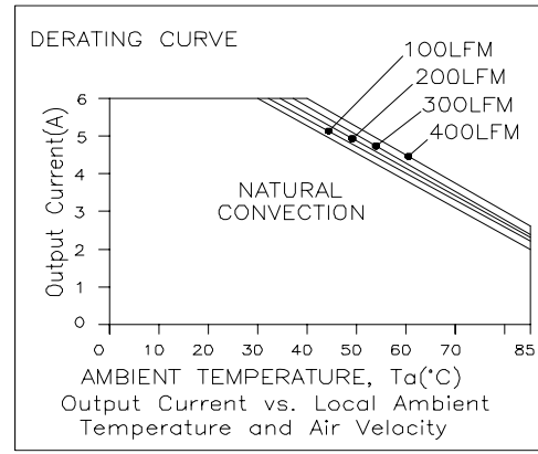
VRBA-06E2Ax, V_o=5.0\text{ V}
