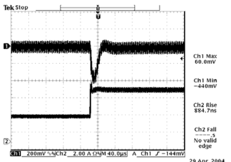
50% to 100% load step at 5.0 V output
