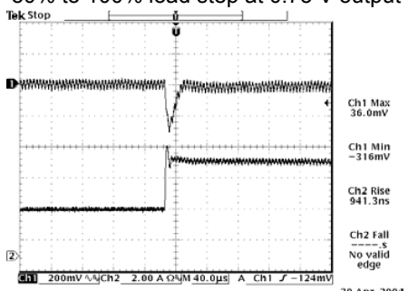
50% to 100% load step at 1.8 V output
