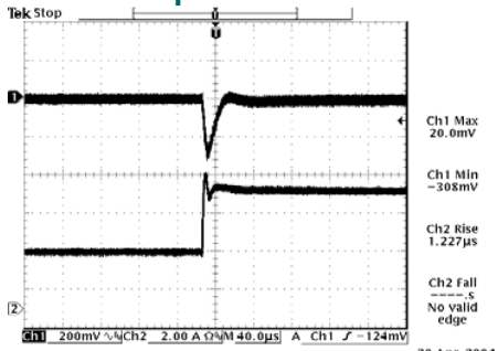
50% to 100% load step at 0.75 V output
