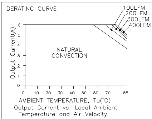
SRBA-06E2Ax, V_o=2.5\text{ V}
