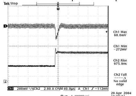
50% to 100% load step at 3.3 V output
