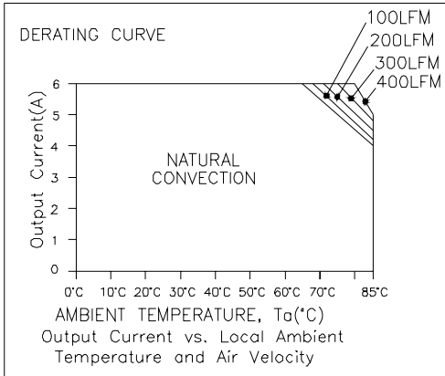
SRBA-06E2Ax, V_o=0.75\text{ V}
