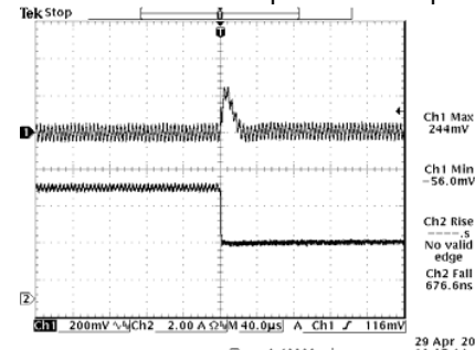
100% to 50% load step at 3.3 V output
