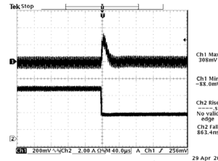
100% to 50% load step at 5.0 V output
