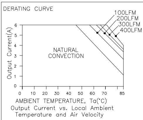
SRBA-06E2Ax, V_o=5.0\text{ V}
