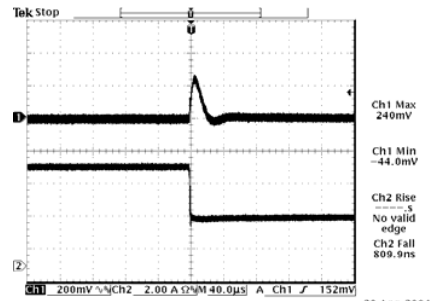
100% to 50% load step at 0.75 V output
