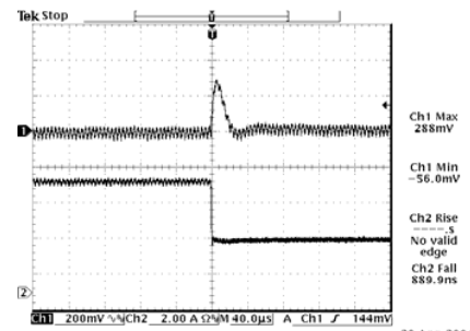
100% to 50% load step at 1.8 V output
