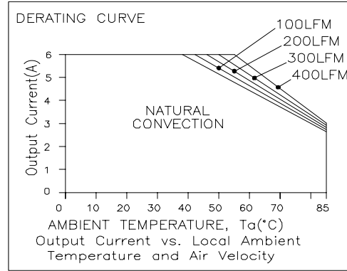
VRBA-06E2Ax, V_o=2.5\text{ V}
