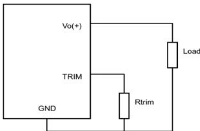
Figure 30: Trim up Circuit configuration for programming output voltage using an external resistor
