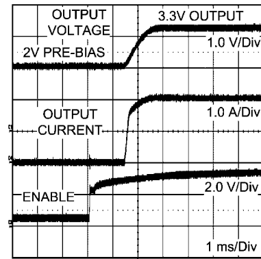
Pre-Biased Startup
