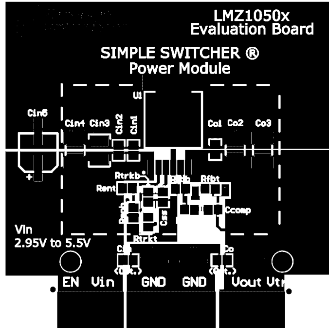
FIGURE 6. Top Copper
