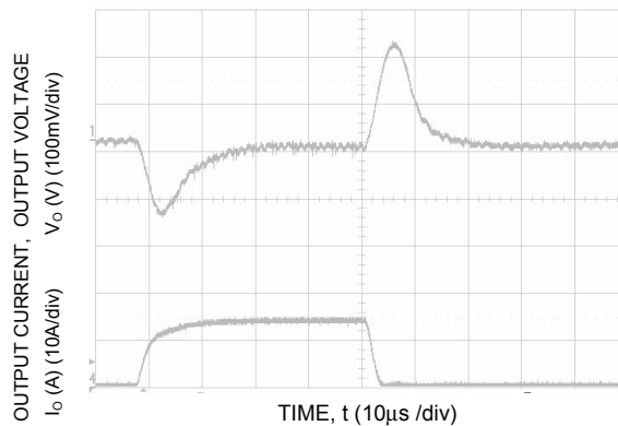
Figure 21. Transient Response to Dynamic Load Change from 0% to 50% to 0% of full load.
