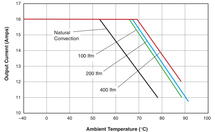
LSN-5/16-D12 Output Current vs. Ambient Temperature (Vertical mount, air flow direction from input pins to output pins)
