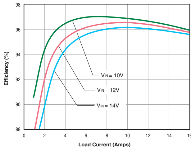
LSN-T/16-D12 Efficiency vs. Line Voltage and Load Current @ 25°C
