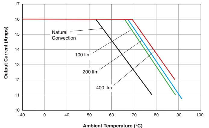
LSN-T/16-D12 Output Current vs. Ambient Temperature (V OUT = 5V, vertical mount, air flow direction from input to output)
