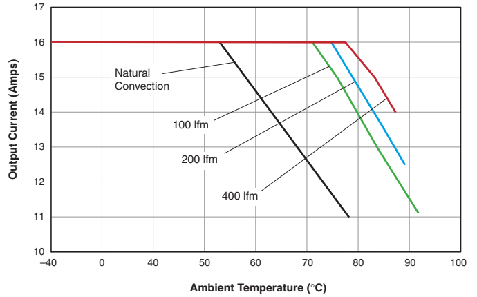
LSN-0.75/16-D12 Output Current vs. Ambient Temperature (Vertical mount, air flow direction from input pins to output pins)
