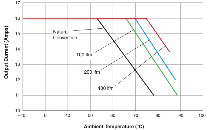
LSN-3.3/16-D12 Output Current vs. Ambient Temperature (Vertical mount, air flow direction from input pins to output pins)
