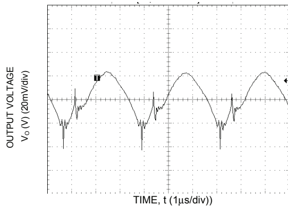
Figure 2. Typical output ripple and noise ( V_{IN} = V_{IN,NOM} , I_o = I_{o,max} ).
