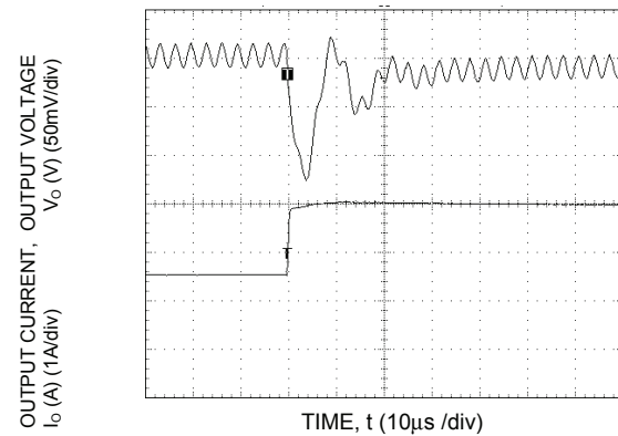
Figure 21. Transient Response to Dynamic Load change from 50% to 100% of full load with di/dt of 5A/µs.
