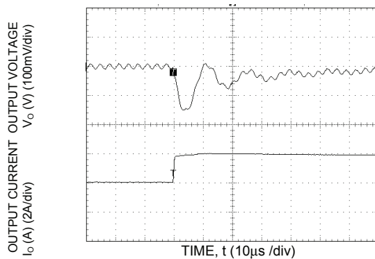
Figure 15. Transient Response to Dynamic Load change from 50% to 100% of full load with di/dt of 5A/\mu s .
