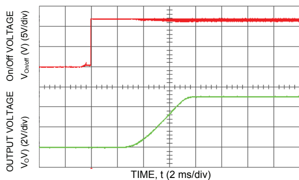
Figure 15. Typical Start-Up Using Remote On/Off with Low-ESR external capacitors ( 7 \times 150\ \mu\text{F} Polymer) ( V_{in} = 12\text{Vdc} , V_o = 5.0\text{Vdc} , I_o = 16\text{A} , C_o = 1050\ \mu\text{F} ).
