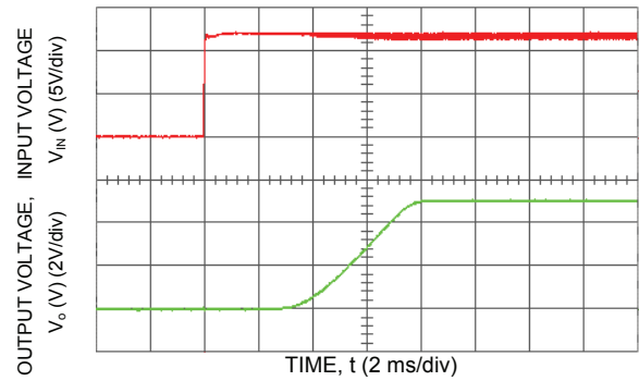
Figure 16. Typical Start-Up with application of V_{in} with low-ESR polymer capacitors at the output ( 7 \times 150\ \mu\text{F} ) ( V_{in} = 12\text{Vdc} , V_o = 5.0\text{Vdc} , I_o = 16\text{A} , C_o = 1050\ \mu\text{F} ).
