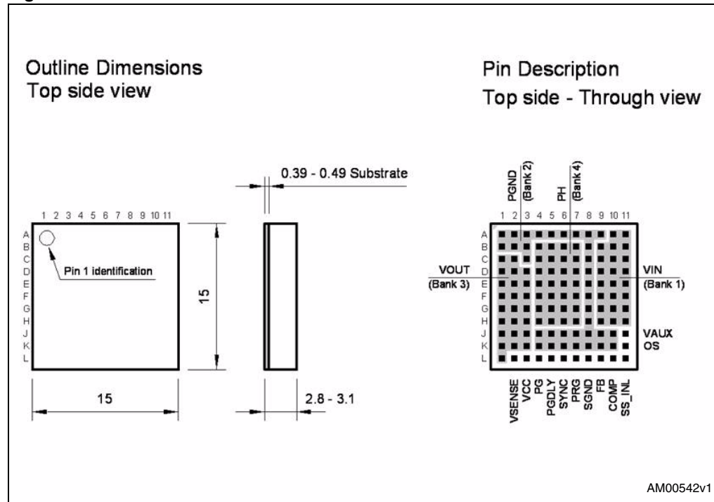
Figure 1. Pin connection
