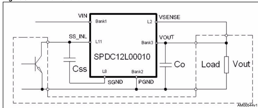
Figure 5. Inhibit function
