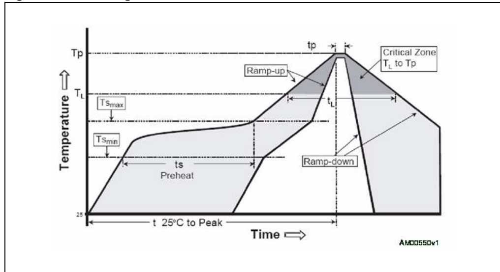
Figure 11. Soldering
