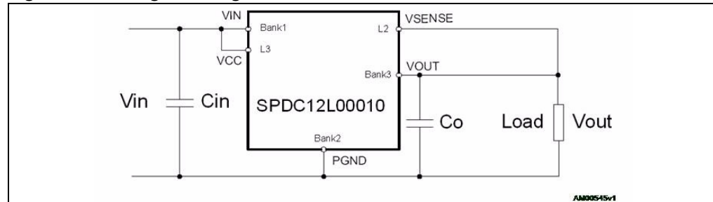
Figure 6. Voltage sensing
