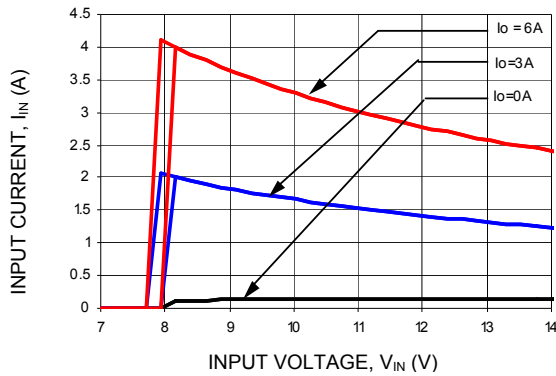
Figure 7. Input voltage vs. Input Current ( V_{out} = 5Vdc ).
