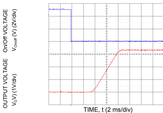
Figure 15. Typical Start-Up Using Remote On/Off with Low-ESR external capacitors ( 7 \times 150\ \mu\text{F} Polymer) ( V_{in} = 5\text{ Vdc} , V_o = 3.3\text{ Vdc} , I_o = 5.0\text{ A} , C_o = 1050\ \mu\text{F} ).
