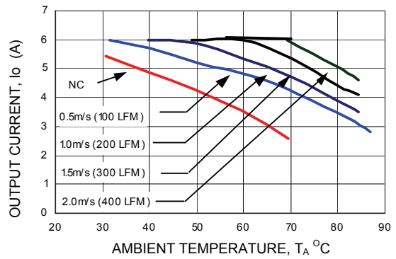
Figure 22. Derating Output Current versus Local Ambient Temperature and Airflow ( V_{in} = 12Vdc , V_o=3.3 Vdc ).
