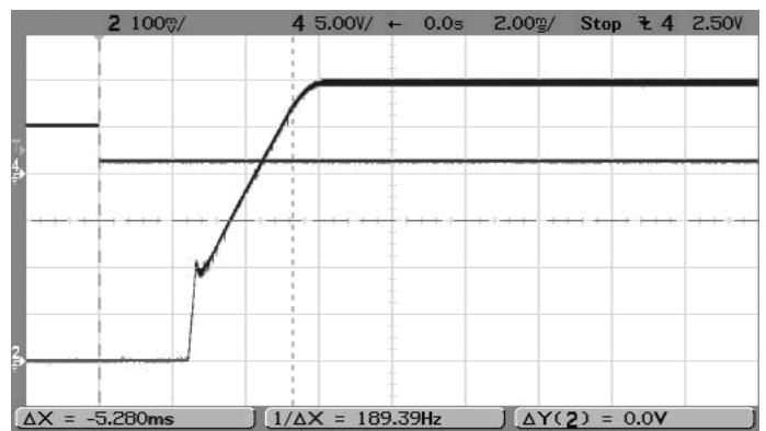
On/Off Enable Startup (V in =5V, V out =0.6V, I out =6A, Cload=0) Trace 4=Enable, Trace 2=V out
