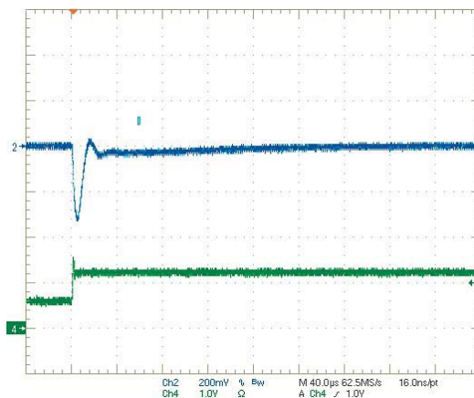
Step Load Transient Response (VIN=5V, V OUT =3.3V, I OUT =3A to 6A) Trace 2=V OUT , 200 mV/div. Trace 4=I OUT , 5A/div.
