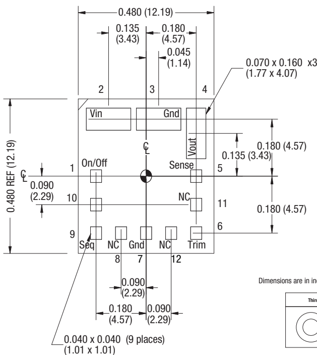
Figure 3. OKL-T/6-W5 Mechanical Outline
