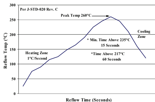
Figure 36. Recommended linear reflow profile using Sn/Ag/Cu solder.
