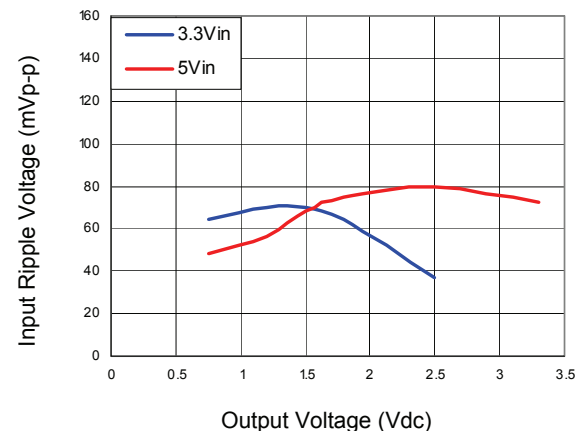
Figure 29. Input ripple voltage for various outputs with 1x47\mu F ceramic capacitor at the input (full load).
