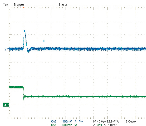
Step Load Transient Response (Vin=5V, Vout=1.2V, Load=0, Iout=3A to 1.5A) Trace 2=Vout, 100 mV/div. Trace 4=Iout, 1A/div.
