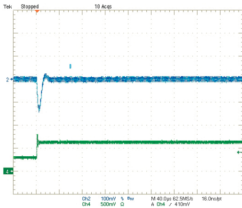
Step Load Transient Response (Vin=5V, Vout=1.8V, Clod=0, Iout=1.5A to 3A) Trace 2=Vout, 100 mV/div. Trace 4=Iout, 1A/div.
