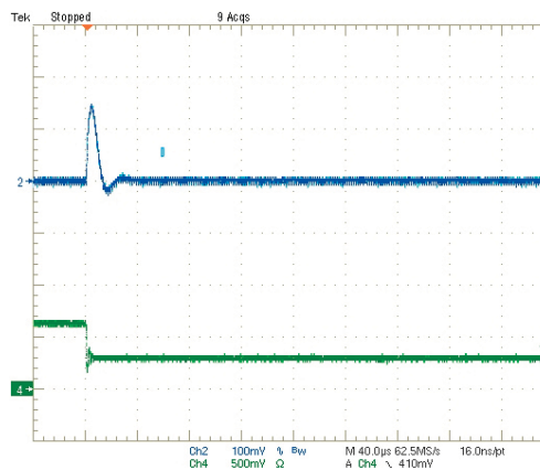
Step Load Transient Response (Vin=5V, Vout=0.6V, Load=0, Iout=3A to 1.5A) Trace 2=Vout, 100 mV/div. Trace 4=Iout, 1A/div.
