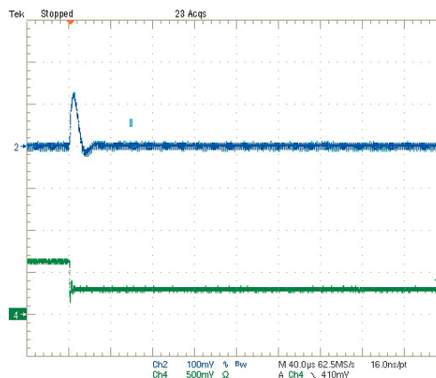
Step Load Transient Response (Vin=5V, Vout=1.0V, Clod=0, Iout=3A to 1.5A) Trace 2=Vout, 100 mV/div. Trace 4=Iout, 1A/div.
