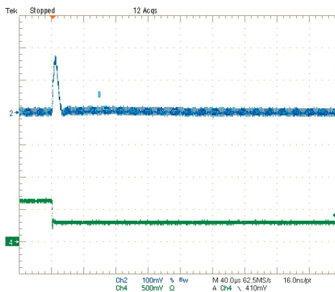
Step Load Transient Response (Vin=5V, Vout=3.3V, Clad=0, Iout=3A to 1.5A) Trace 2=Vout, 100 mV/div. Trace 4=Iout, 1A/div.
