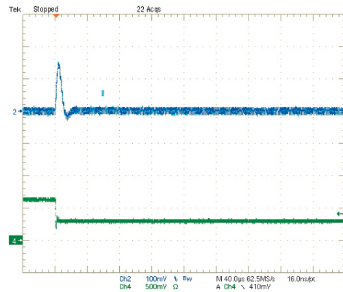
Step Load Transient Response (Vin=5V, Vout=1.8V, Clod=0, Iout=3A to 1.5A) Trace 2=Vout, 100 mV/div. Trace 4=Iout, 1A/div.
