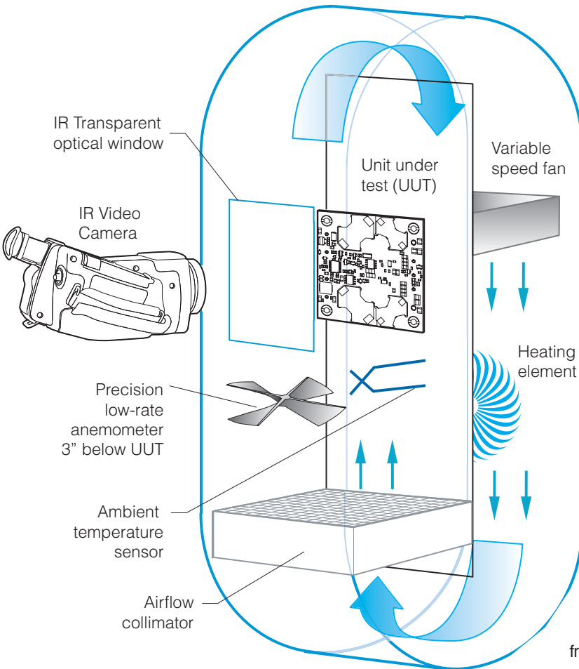
Figure 6. Vertical Wind Tunnel
