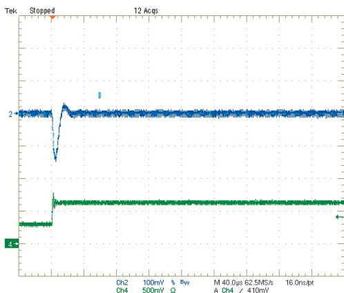
Step Load Transient Response (Vin=5V, Vout=1.2V, Load=0, Iout=1.5A to 3A) Trace 2=Vout, 100 mV/div. Trace 4=Iout, 1A/div.
