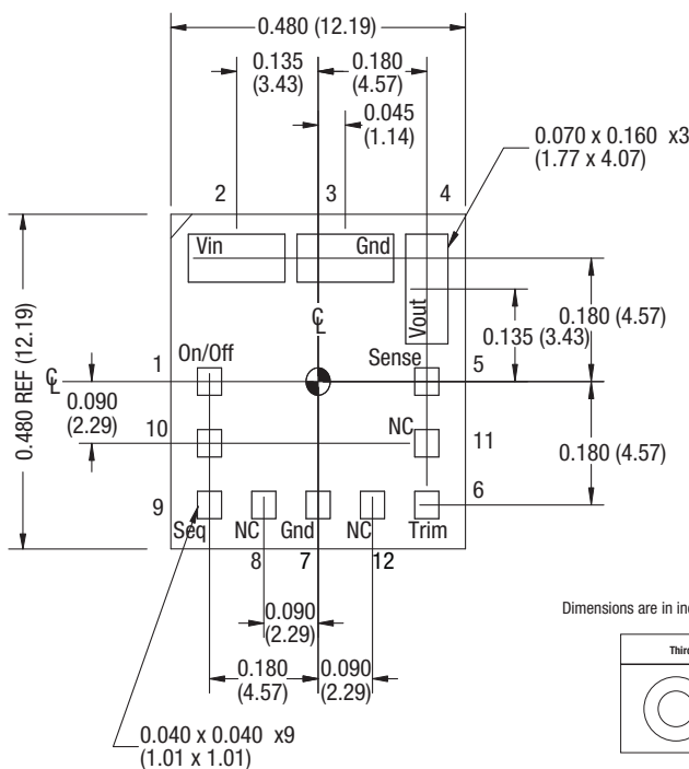
Figure 3. OKL-T/3-W5 Mechanical Outline
