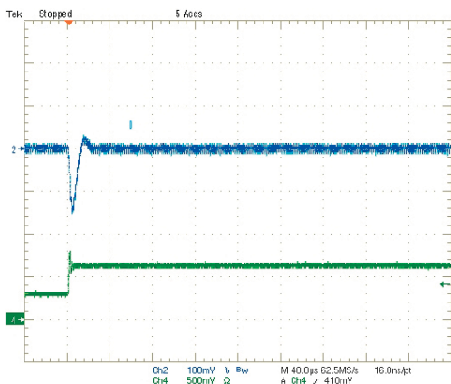
Step Load Transient Response (Vin=5V, Vout=1.5V, Load=0, Iout=1.5A to 3A) Trace 2=Vout, 100 mV/div. Trace 4=Iout, 1A/div.
