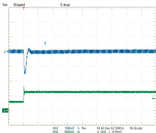
Step Load Transient Response (Vin=5V, Vout=2.5V, Clod=0, Iout=1.5A to 3A) Trace 2=Vout, 100 mV/div. Trace 4=Iout, 1A/div.
