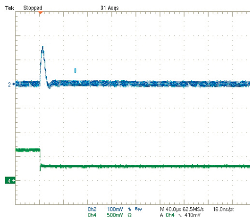
Step Load Transient Response (Vin=5V, Vout=2.5V, Clod=0, Iout=3A to 1.5A) Trace 2=Vout, 100 mV/div. Trace 4=Iout, 1A/div.
