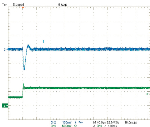
Step Load Transient Response (Vin=5V, Vout=1.0V, Clod=0, Iout=1.5A to 3A) Trace 2=Vout, 100 mV/div. Trace 4=Iout, 1A/div.
