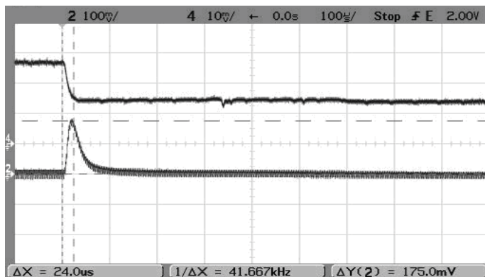
Step Load Transient Response (Vin=5V, Vout=3.3V, Load=0, Iout=5A to 2.5A) Trace 2=Vout, 100 mV/div. Trace 4=Iout, 2A/div.
