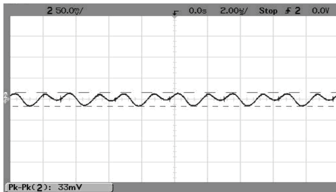
Output Ripple and Noise (Vin=5V, Vout=3.3V, Iout=5A, Load=0, ScopeBW=100MHz)
