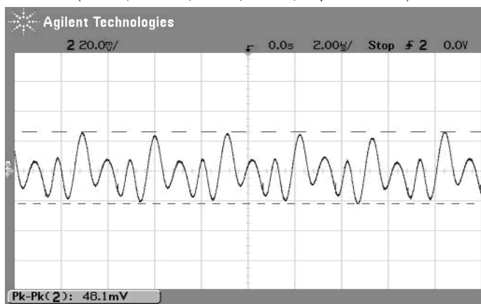
Output Ripple and Noise (Vin=12V, Vout=1.2V, Iout=3A, Load=0, ScopeBW=100MHz)
