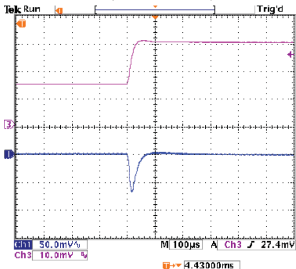
Step Load Transient Response (Vin=12V, Vout=1.2V, Load=0, Iout=1.5A to 3A) Trace 1=Vout, 50 mV/div. Trace 3=Iout, 1A/div.
