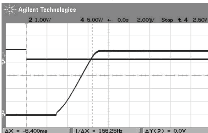
On/Off Enable Startup Delay (Vin=12V, Vout=5V, Iout=5A, Clod=0 Trace 4=Enable In, Trace2=Vout)
