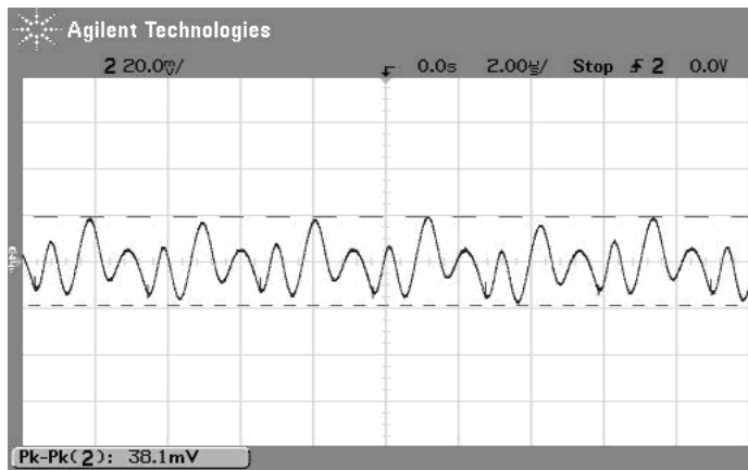
OKY-T/3-D12 Output Ripple and Noise (VIN=12V, Vout=0.75V, Iout=3A, Clload=0, ScopeBW=100MHz)
