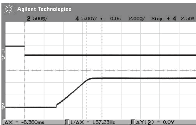
On/Off Enable Startup Delay (Vin=12V, Vout=1.2V, Iout=3A, Load=0) Trace 4=Enable In, Trace2=Vout
