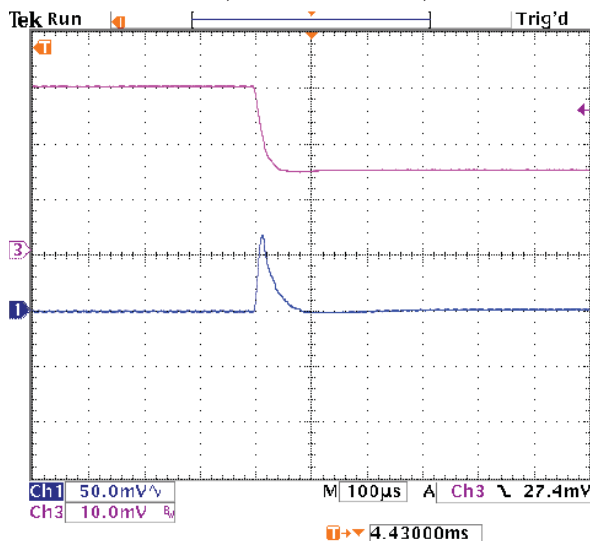
Step Load Transient Response (Vin=12V, Vout=1.2V, Load=0, Iout=3A to 1.5A) Trace 1=Vout, 50 mV/div. Trace 3=Iout, 1A/div.
