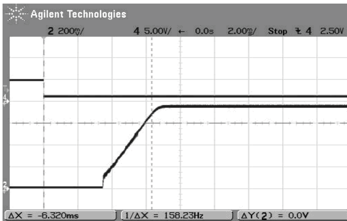
On/Off Enable Startup Delay (VIN=12V, Vout=0.75V, Iout=3A, Clload=0) Trace 4=Enable In, Trace2=Vout
