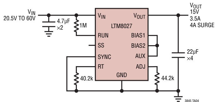
15V V_{OUT} Step-Down Converter
