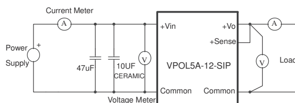
Figure 11. VPOL5A-12-SIP Test Setup
