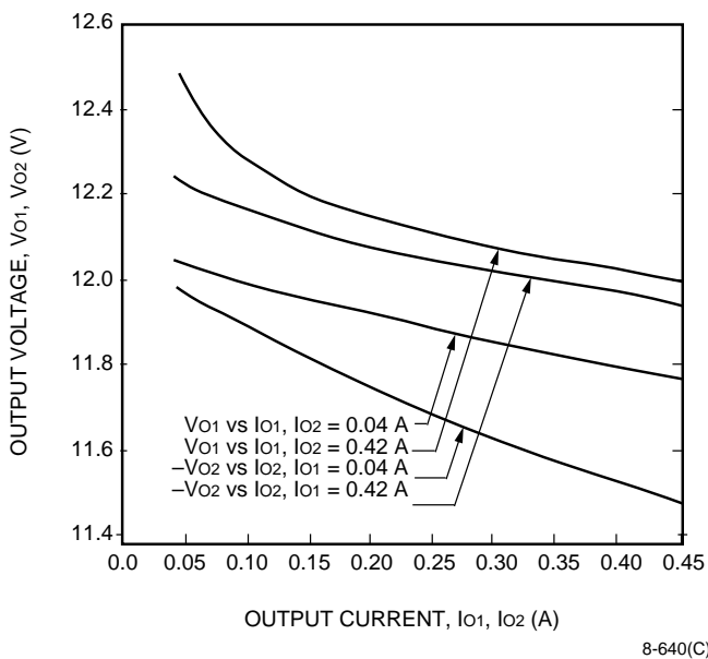
Figure 2. MW010BK Typical Output Voltage Regulation; T_A = 25^\circ\text{C} ; V_i = 48 \text{ V}
