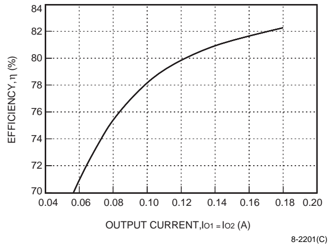
Figure 24. ME005CL Typical Converter Efficiency as a Function of Output Current with V_i = 48\text{ V} and T_A = 25\text{ °C}
