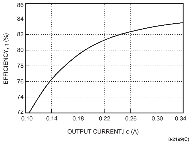
Figure 22. ME005C Typical Converter Efficiency as a Function of Output Current with V_i = 48\text{ V} and T_A = 25\text{ °C}
