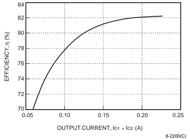
Figure 23. ME005BK Typical Converter Efficiency as a Function of Output Current with V_i = 48\text{ V} and T_A = 25\text{ °C}
