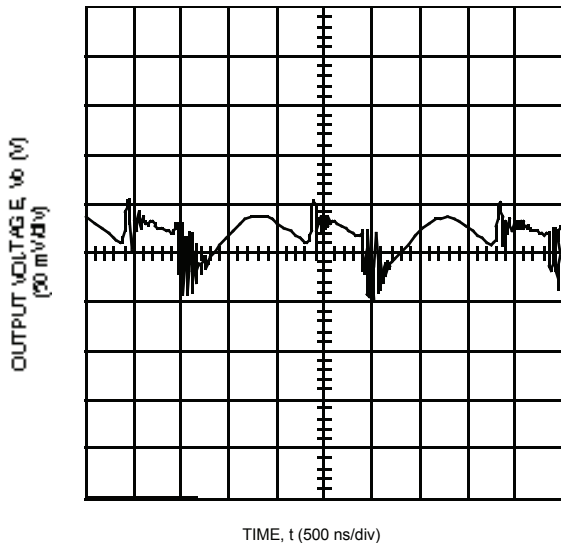
Figure 13. Typical JW150D Output Ripple Voltage at Room Temperature, 48 V Input, I_o = I_{o, max}
